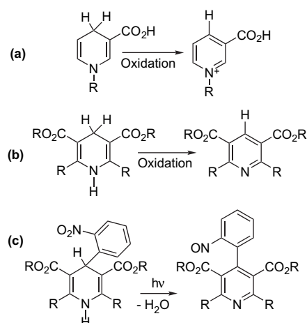
Scheme 1. Dihydropyridine–pyridine (or pyridinium ion) reactions and photochemistry of a nitrophenyldihydropyridine.
