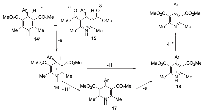
Scheme 3. Suggested mechanism for the photochemistry of dihydropyridines (general formula 14 ).
