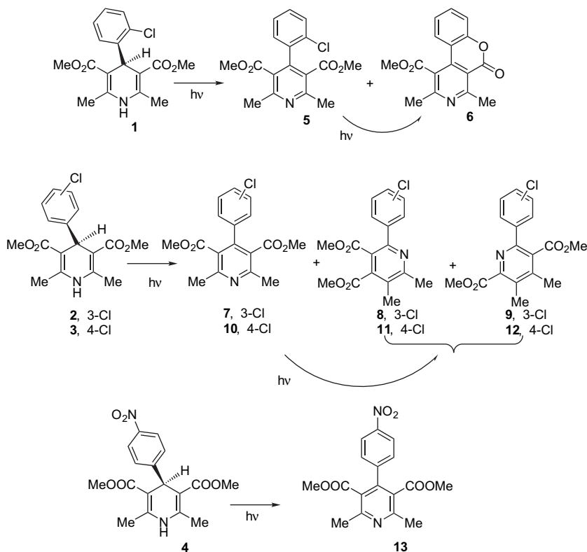
Scheme 2. Photoproducts from dihydropyridines 1 – 4 .
