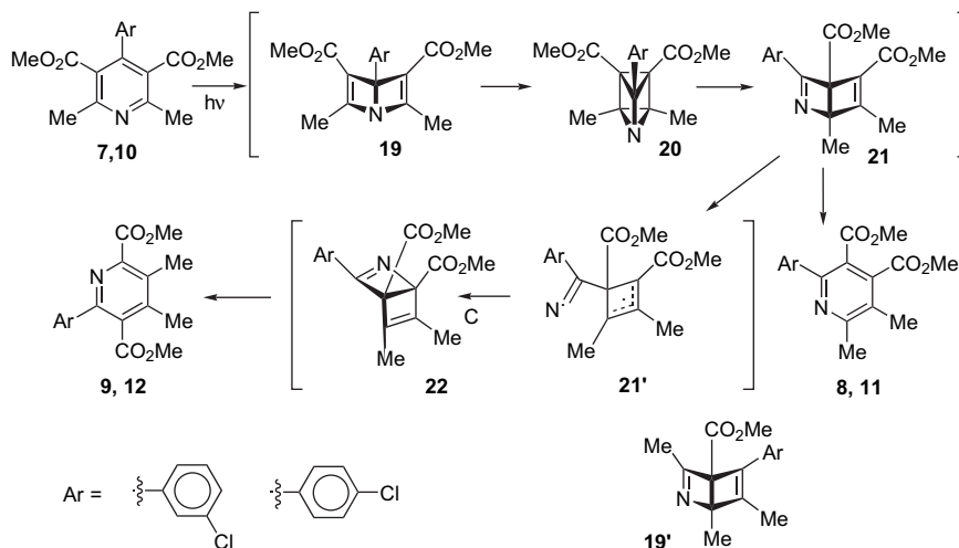
Scheme 5. Photorearrangement of pyridines 7 and 10 .
