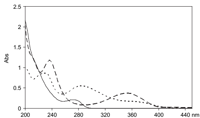
Figure 1. Absorption spectrum of dihydropyridine 1 (---), of the corresponding pyridine 5 (—) and of the compound 4 (...), 5 \times 10^{-5} \text{ M} in acetonitrile.
