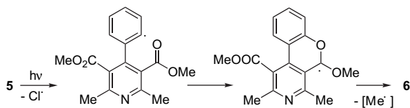
Scheme 4. Photochemical reaction of pyridine 5 .
